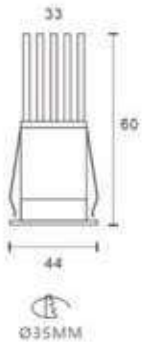
D8005L LED 8W
