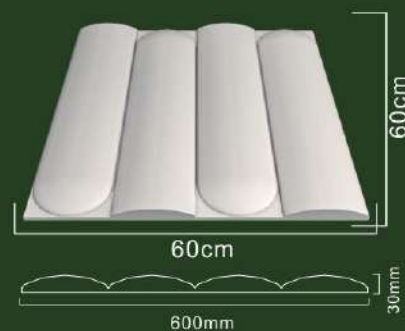
K4175 size: 60x60x3cm (23 5/8" x 23 5/8" x 1 3/16")
