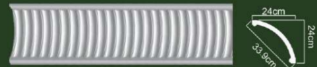
AA376A size:244x24x24cm (96 1/16 " x9 7/16 " x9 7/16 " )
