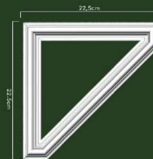
B5017 outside: \Phi 22.5\text{cm} (8 7/8") thickness: 1.4cm (9/16")
