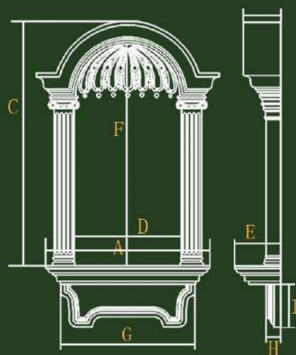
K6010 + size: 53.7x86x15cm A:53.7cm (21 1/8 ") B:11cm (4 5/16 ") C:86cm (33 7/8 ") D:35cm (13 3/4 ") E:15cm (5 15/16 ") F:72.5cm (28 1/2 ")
