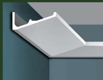
AB319 size:240x20x8cm (94 1/2 " x7 7/8 " x3 1/8 " )
