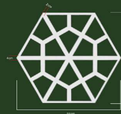
B5014 size: 98x85x1.5cm (38 9/16" x 33 1/2" x 5/8")
