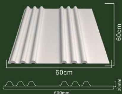
K4173 size: 60x60x3cm (23 5/8" x 23 5/8" x 1 3/16")
