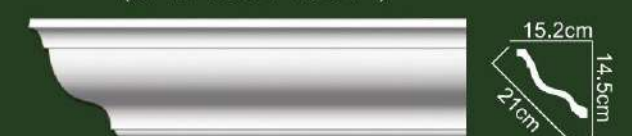
AB214 size:244x14.5x15.2cm (96 1/16 " x5 11/16 " x6 " )
