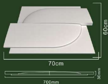
K4177 size: 70x60x3cm (27 1/4" x 23 5/8" x 1 3/16")
