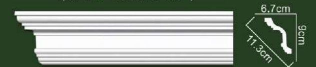
AB215 size:244x9x6.7cm (96 1/16 " x3 1/2 " x2 5/8 " )
