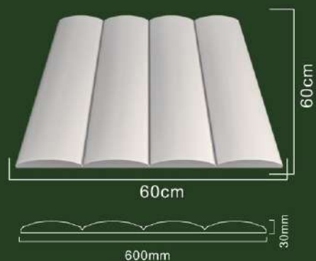
K4176 size: 60x60x3cm (23 5/8" x 23 5/8" x 1 3/16")
