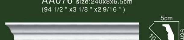
AA077 size:240x9x5cm (94 1/2 " x3 9/16 " x1 15/16 " )
