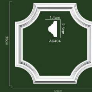
B5015 outside: \Phi 30\text{cm} (11 13/16") thickness: 1.4cm (9/16")
