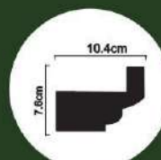
AD474B size:240x7.6x10.4cm (94 1/2"x3"x4 1/8")
