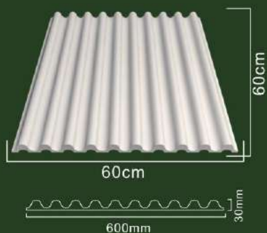
K4174 size: 60x60x3cm (23 5/8" x 23 5/8" x 1 3/16")
